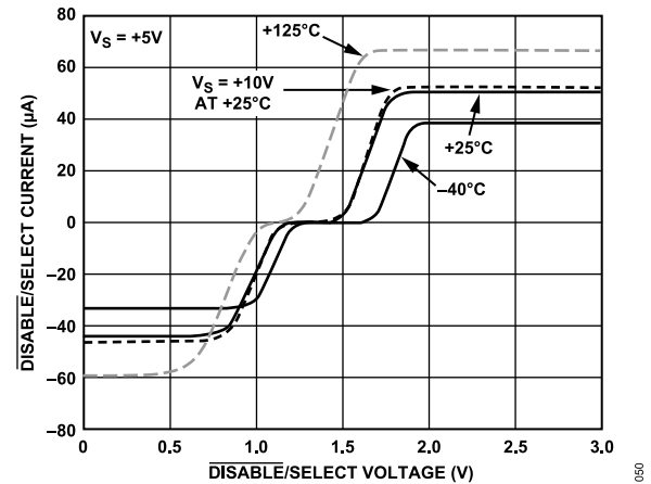
Figure 55. \overline{DISABLE}/SELECT Current vs. \overline{DISABLE}/SELECT Voltage and Temperature
