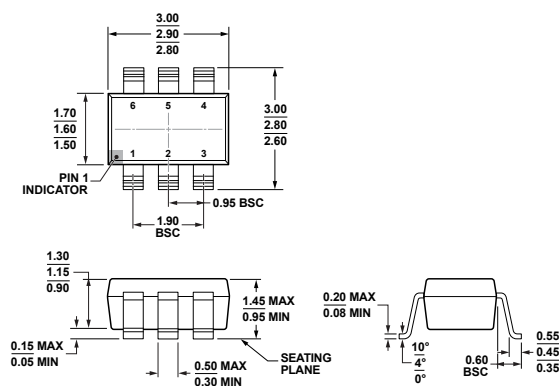
Figure 69. 8-Lead Standard Small Outline Package [SOIC_N] Narrow Body (R-8) Dimensions shown in millimeters and (inches)
