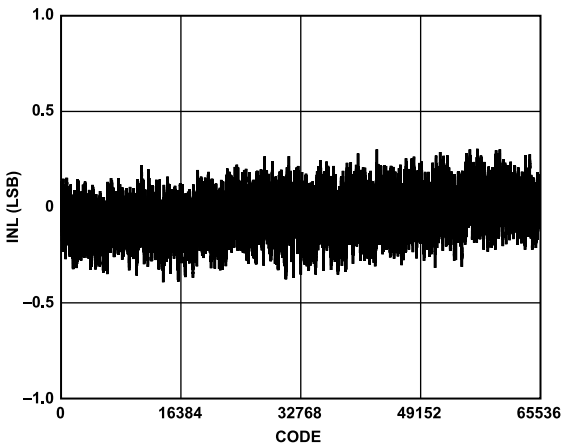
Figure 66. Integral Nonlinearity
