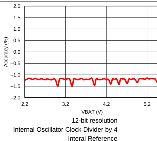
Figure 12. Battery Measurement, Accuracy versus VBAT Input Voltage
