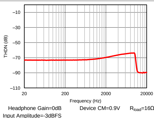
Figure 28. DAC Playback on Headphone Amplifier, Total Harmonic Distortion + Noise versus Input Frequency
