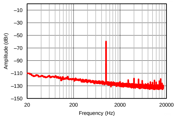
Figure 25. DAC Playback on Headphone Amplifier, Output Amplitude versus Frequency
