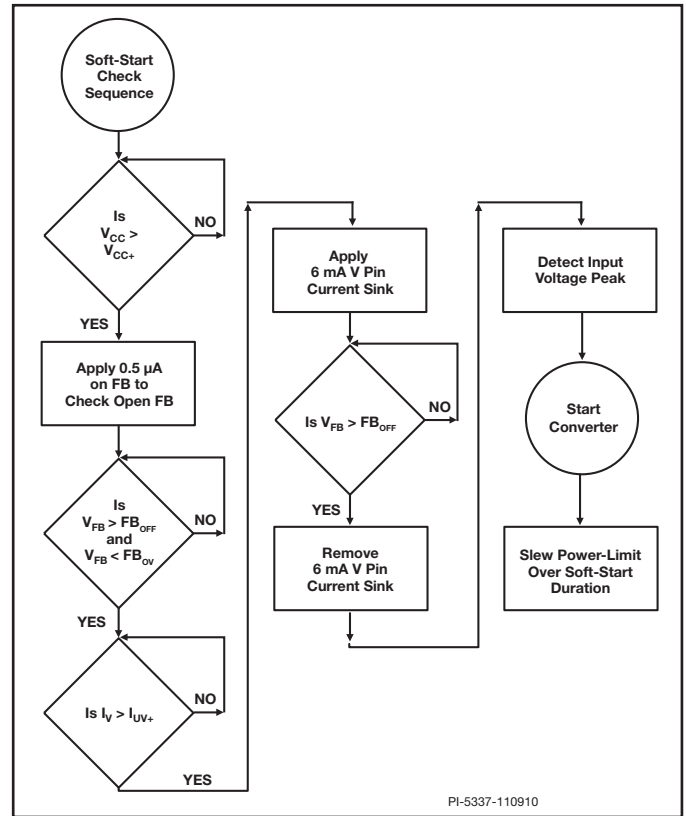
Figure 7. Start-Up Sequence.
