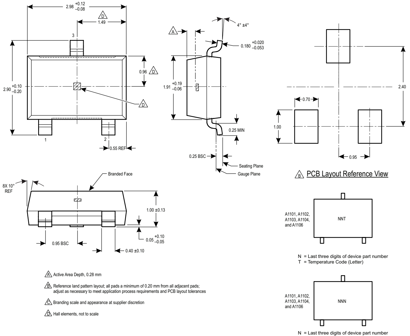
Figure 3: Package LH, 3-Pin (SOT-23W)
