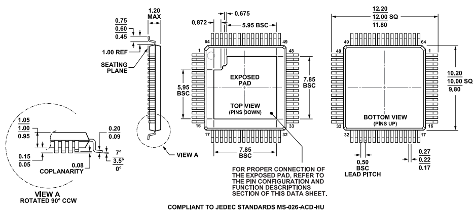
Figure 64. 64-Lead Thin Quad Flat Package, Exposed Pad [TQFP_EP] (SV-64-3)
