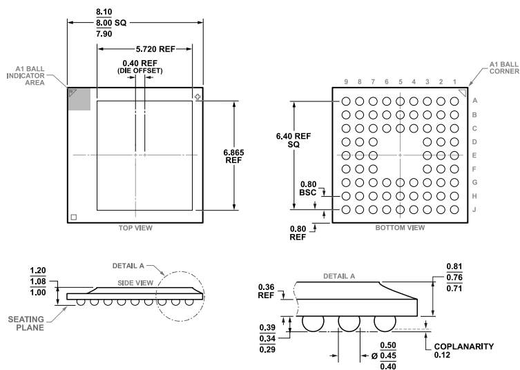
Figure 65. 72-Ball Chip Scale Package Ball Grid Array [CSP_BGA] (BC-72-2)
