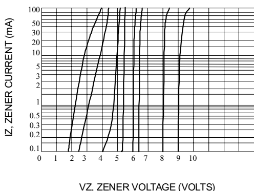
Fig. 6-VZ = 3.9 THRU 10 VOLTS
