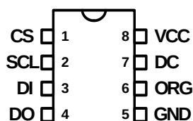
8L PDIP
