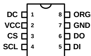
8L SOIC Rotated (R) 93C46 only
