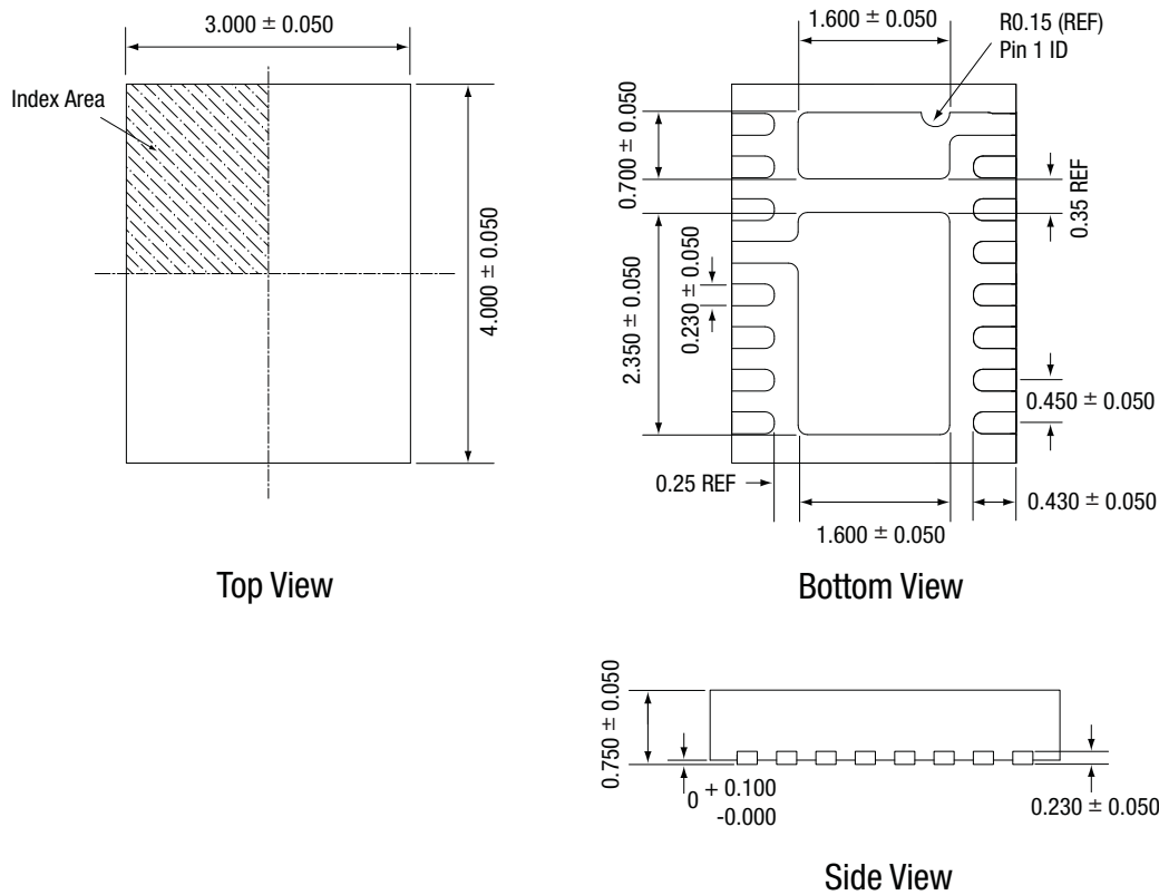
Figure 30. AAT3783A 16-pin TDFN Package Dimensions
