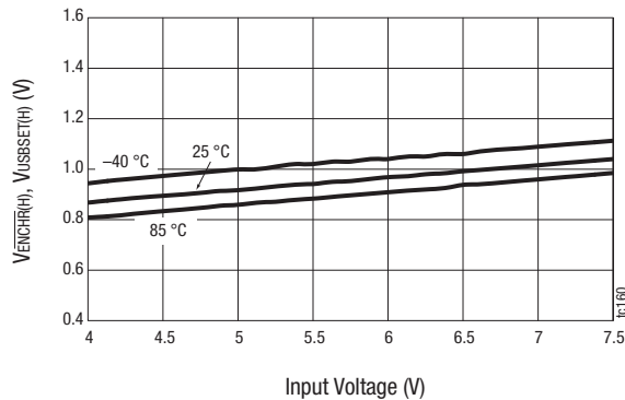
Figure 20. Input High Threshold vs Input Voltage
