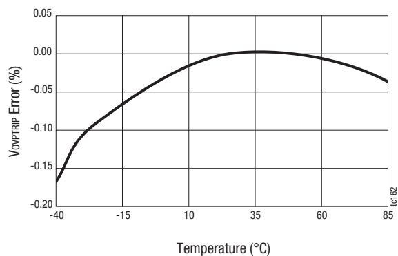
Figure 22. OVP Trip Point vs Temperature
