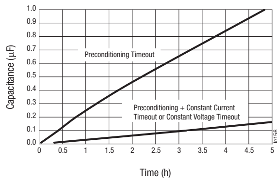
Figure 16. CT Pin Capacitance vs Counter Timeout
