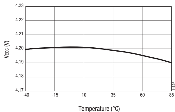
Figure 6. End of Charge Voltage vs Temperature
