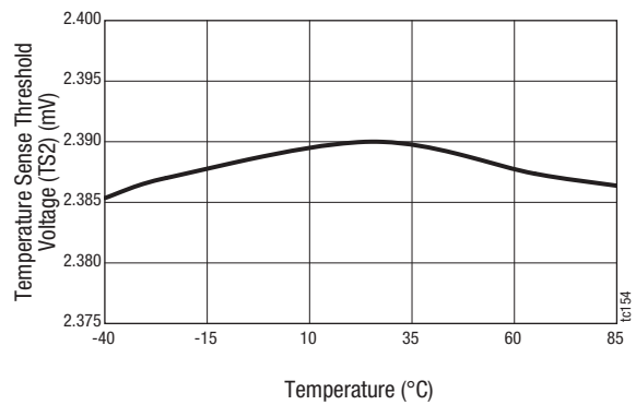
Figure 14. Temperature Sense too Cold Threshold vs Temperature
