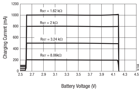
Figure 4. Battery Charging Current vs Battery Voltage
