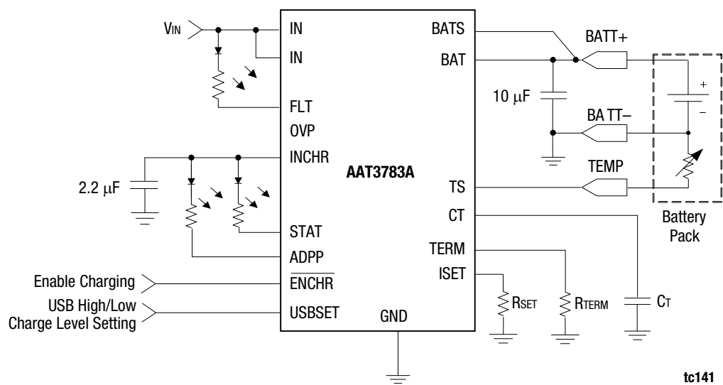
Figure 1. AAT3783A Typical Application Circuit
