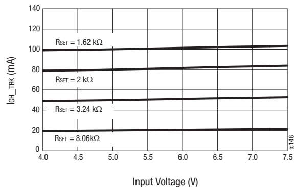
Figure 8. Preconditioning Charge Current vs Input Voltage
