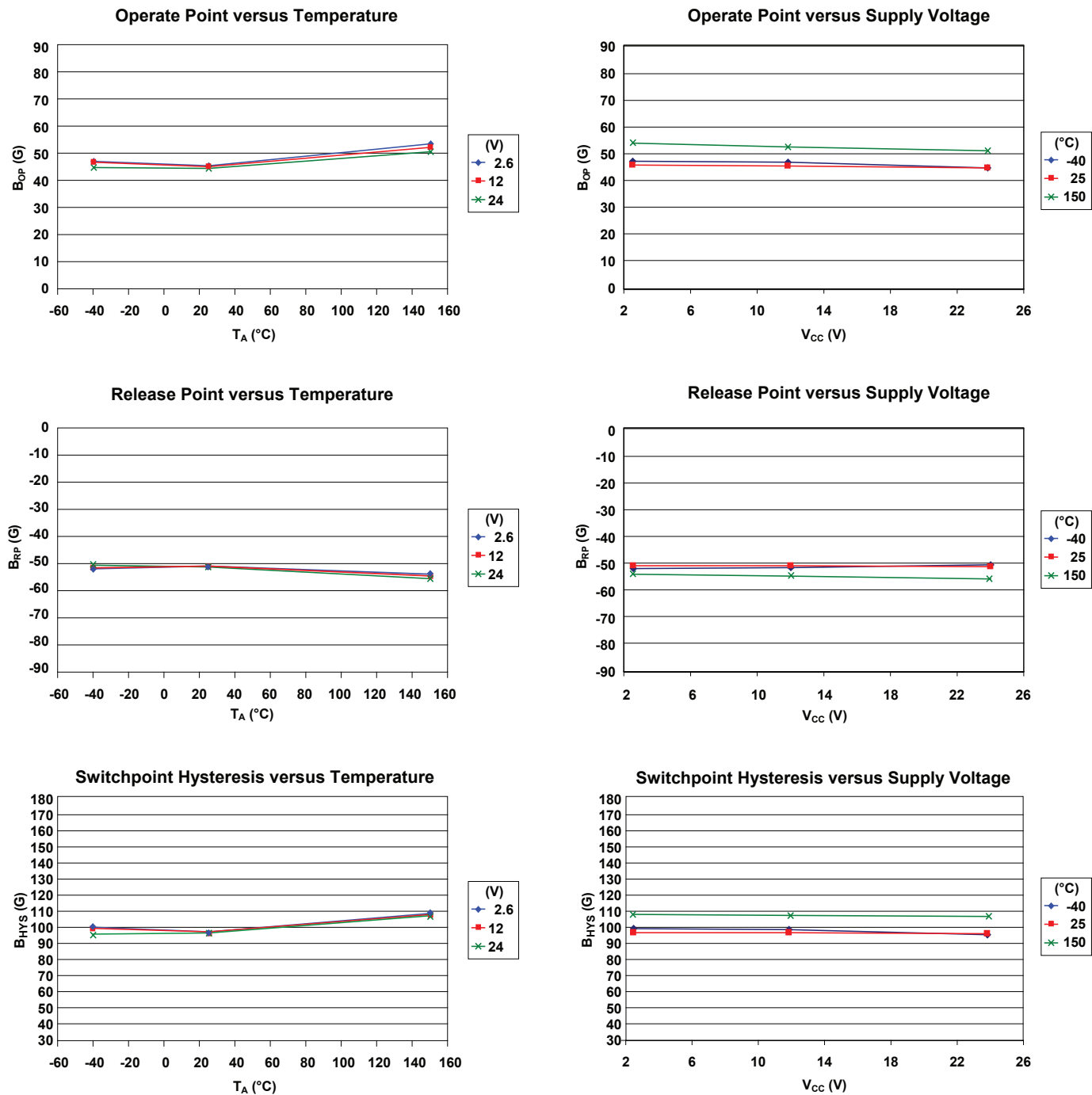
A1221 Magnetic Characteristics
