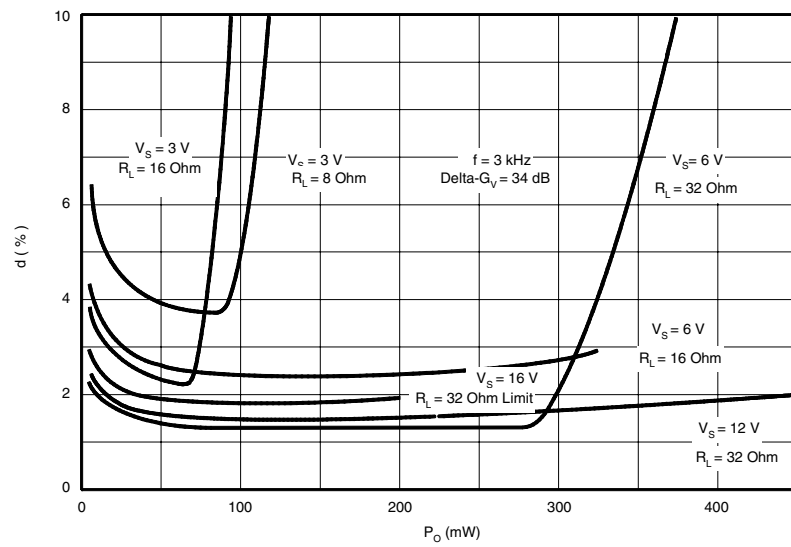
Figure 8-12. Distortion versus Power — f = 3 kHz, \Delta - G_V = 34 dB
