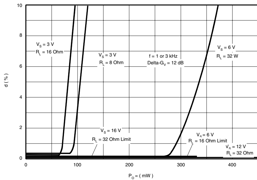
Figure 8-13. Distortion versus Power — f = 1 kHz or 3 kHz, \Delta - G_V = 12 dB
