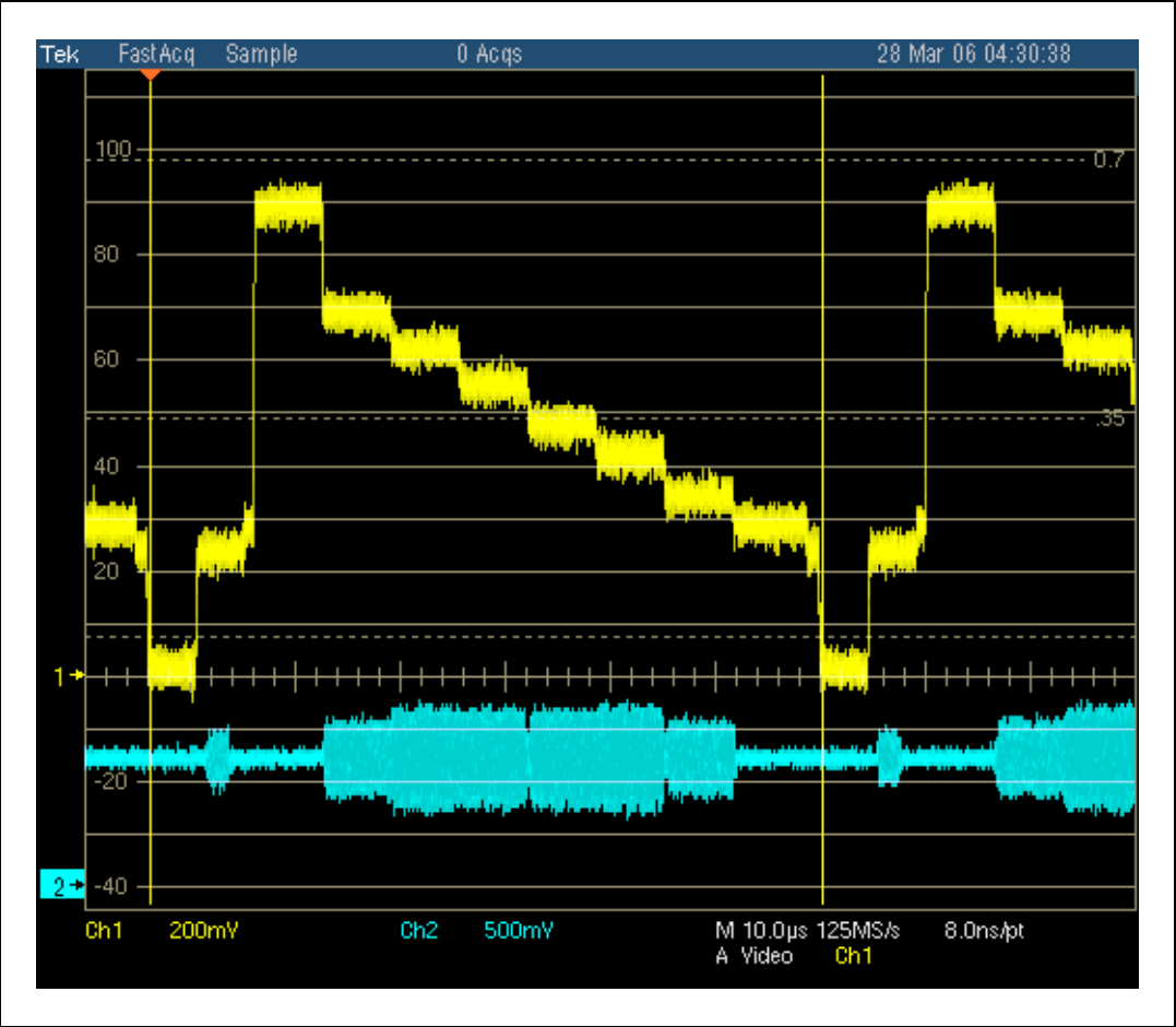
Figure 27. PAL S-video
