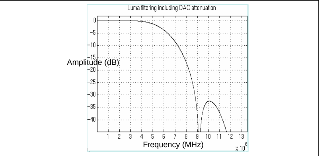
Figure 10. Luma filtering
