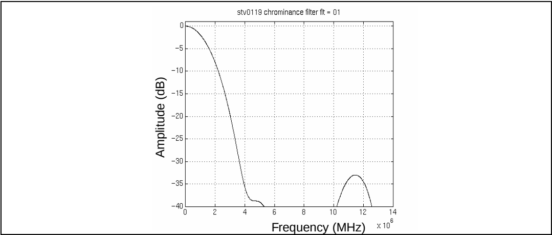
Figure 14. 1.3 MHz chroma filter
