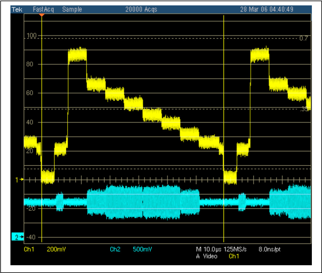
Figure 25. NTSC S-video
