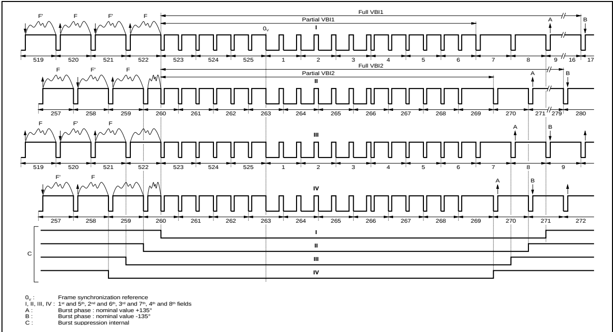
Figure 8. PAL-M typical VBI waveforms, interlaced mode (ITU-R/CCIR-525 line numbering)
