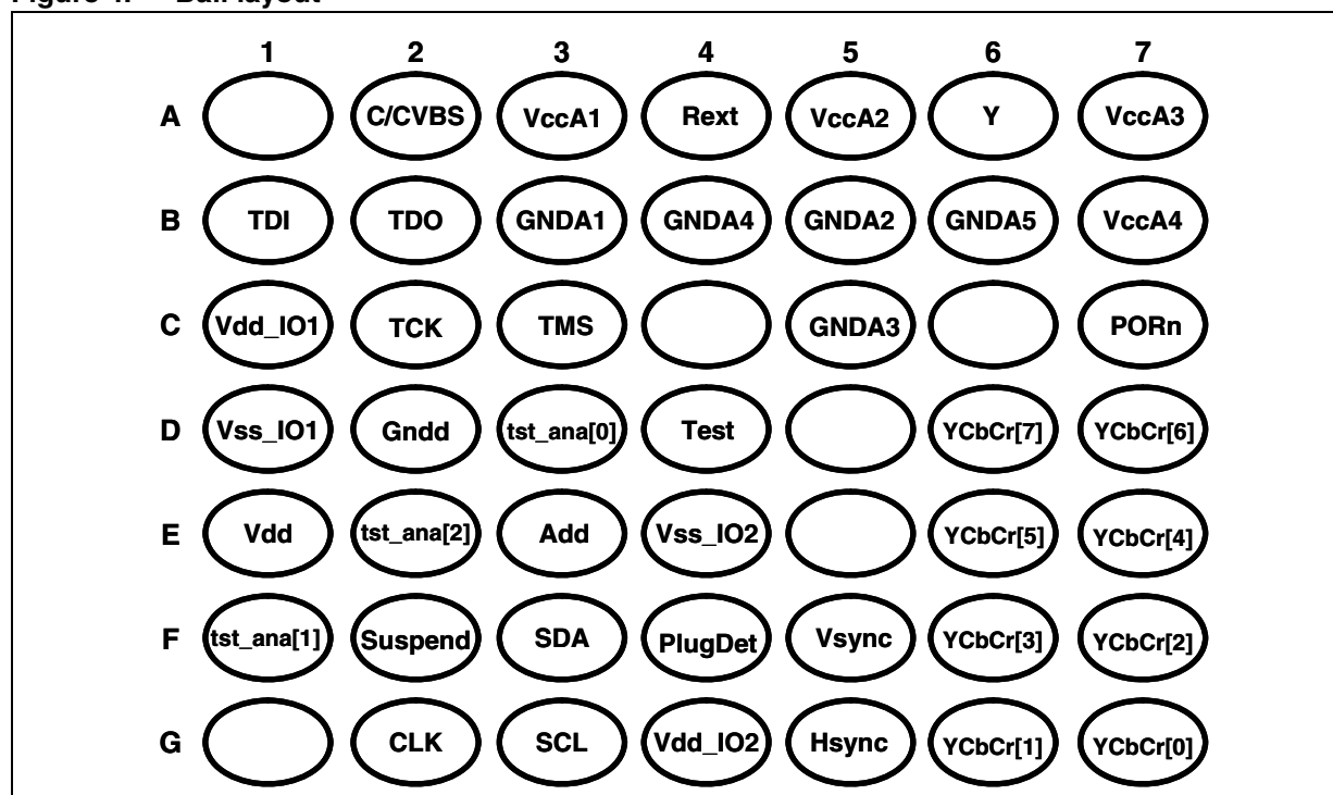
Figure 4. Ball layout
