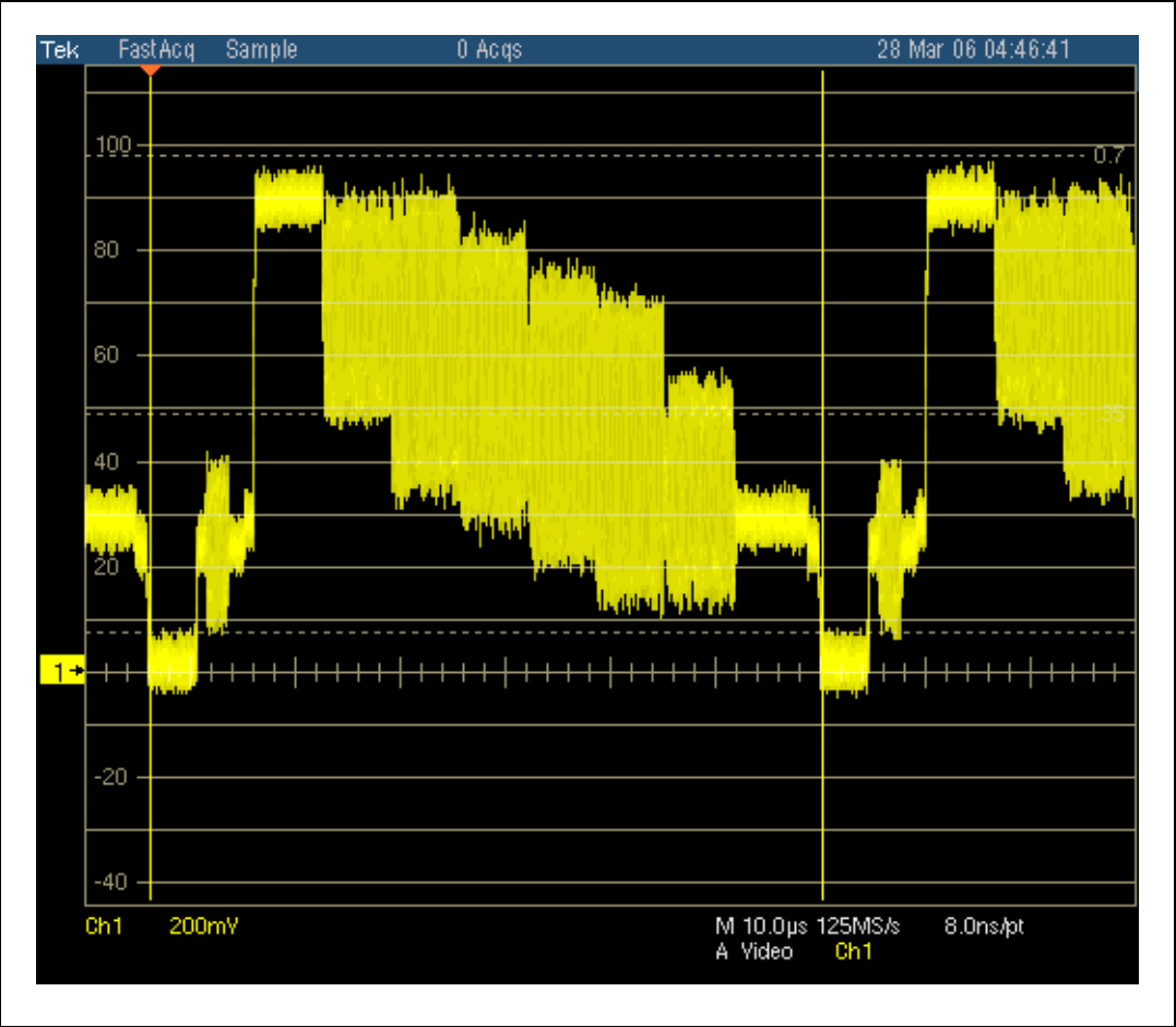
Figure 26. PAL composite
