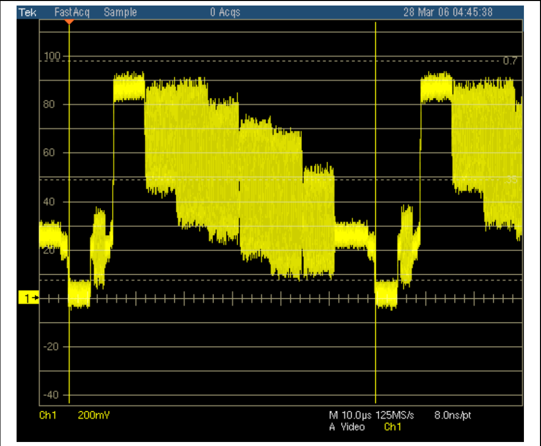
Figure 24. NTSC composite
