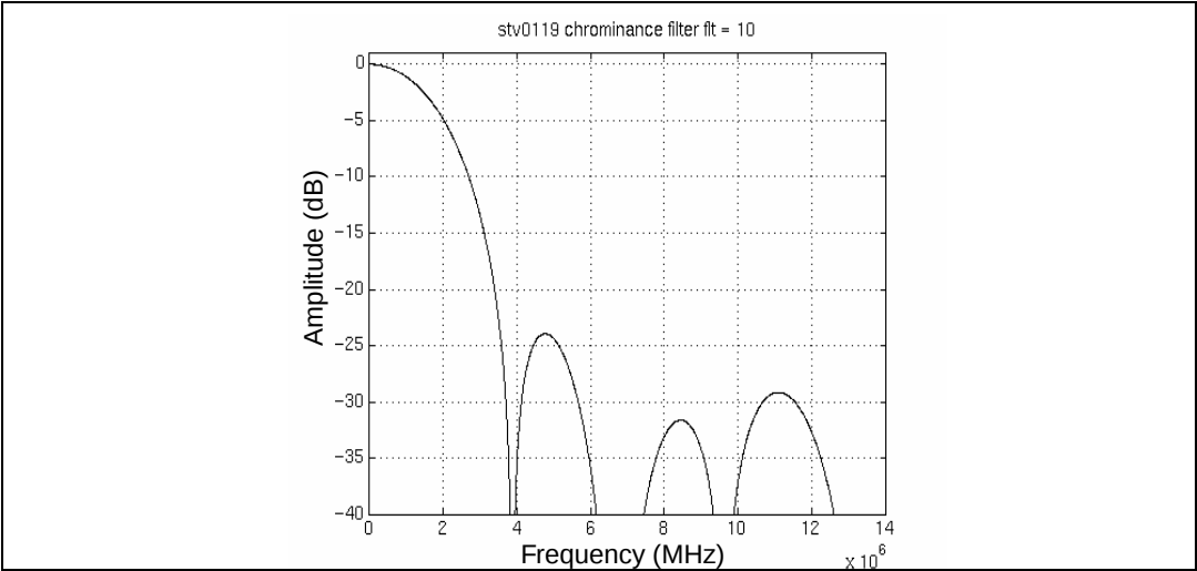
Figure 15. 1.6 MHz chroma filter
