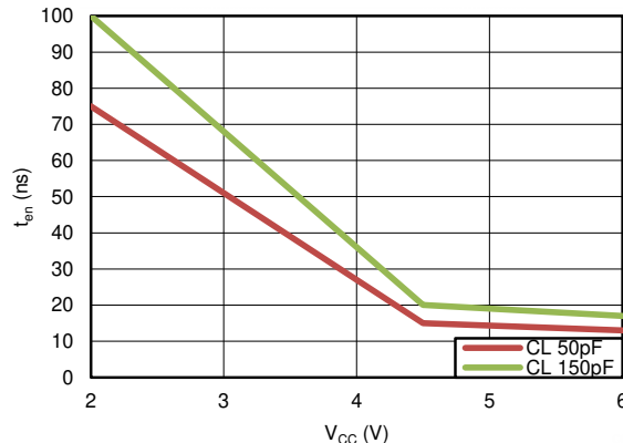
Figure 9-2. Enable Time
