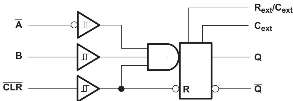
Logic Diagram, Each Multivibrator (Positive Logic)
