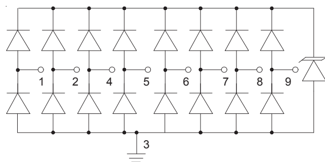
8-Line Protection
