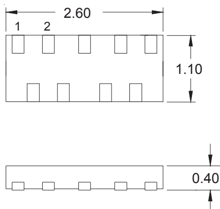
Nominal Dimensions in mm (Bottom View)
