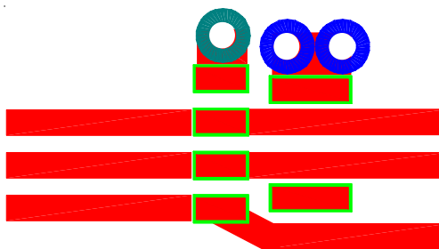
Figure 2 - Layout Example
