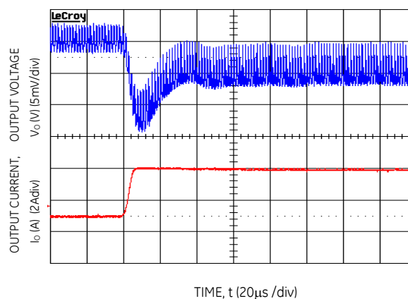
Figure 4. Transient Response to Dynamic Load Change from 50% to 100% at 9Vin, C_{out}=2\times 47\mu\text{F}+4\times 330\mu\text{F} , C_{Tune}=33\text{nF} , R_{Tune}=178
