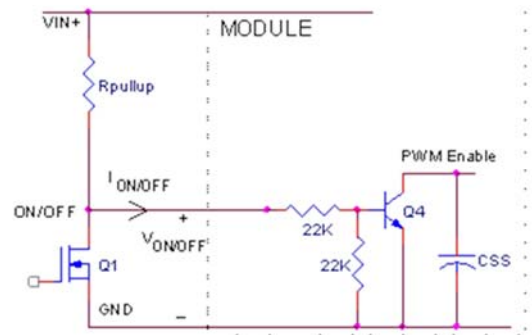
Figure 40. Circuit configuration for using negative On/Off logic.
