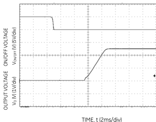
Figure 23. Typical Start-up Using On/Off Voltage ( I_o = I_{o,max} ).
