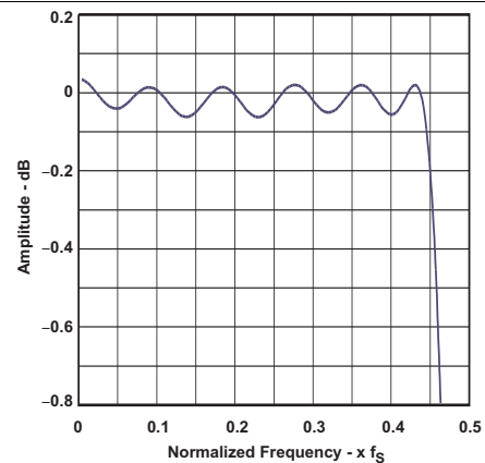
Figure 10. Passband Ripple
