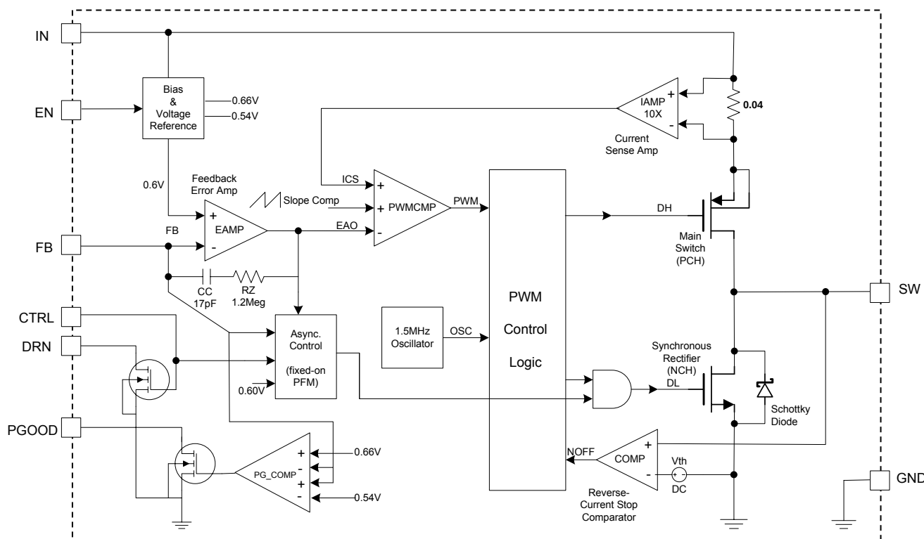
Figure 1-Functional Block Diagram
