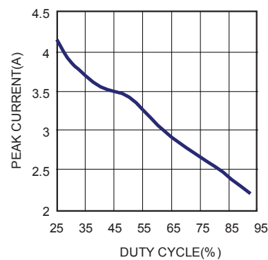
Peak Current vs. Duty
