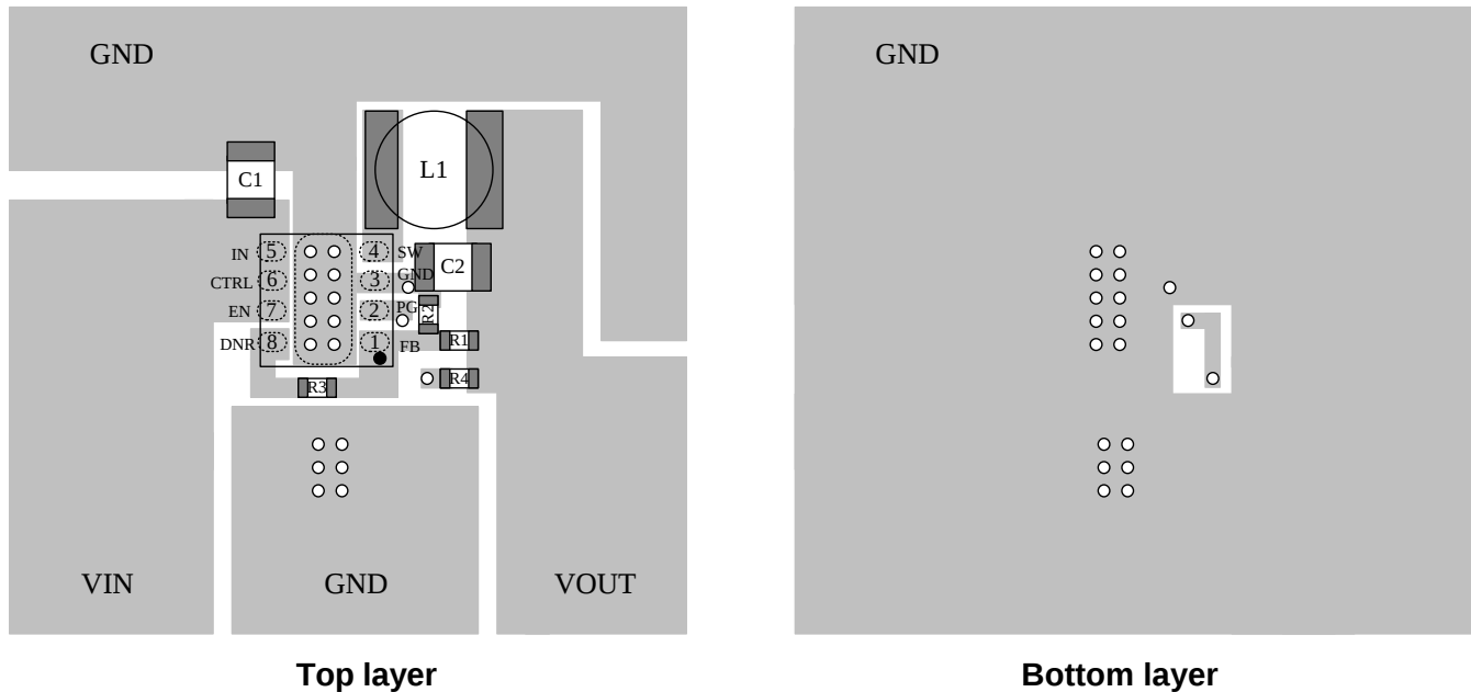
Figure 2-PCB Layout
