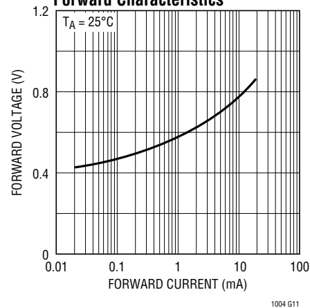
Forward Characteristics
