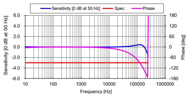
Figure 7: Frequency response
