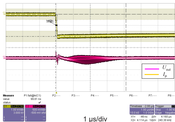
Figure 14: dv/dt
