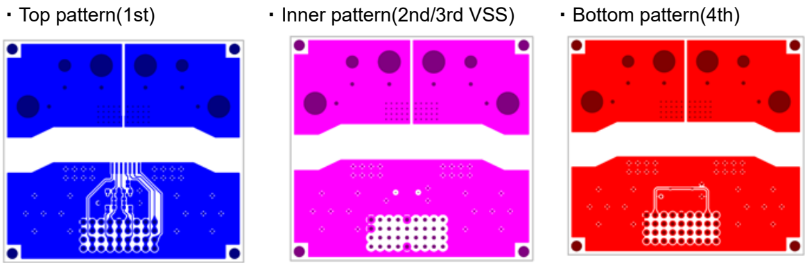
Figure 7. Board layout for measuring thermal resistance of CZ-3704
