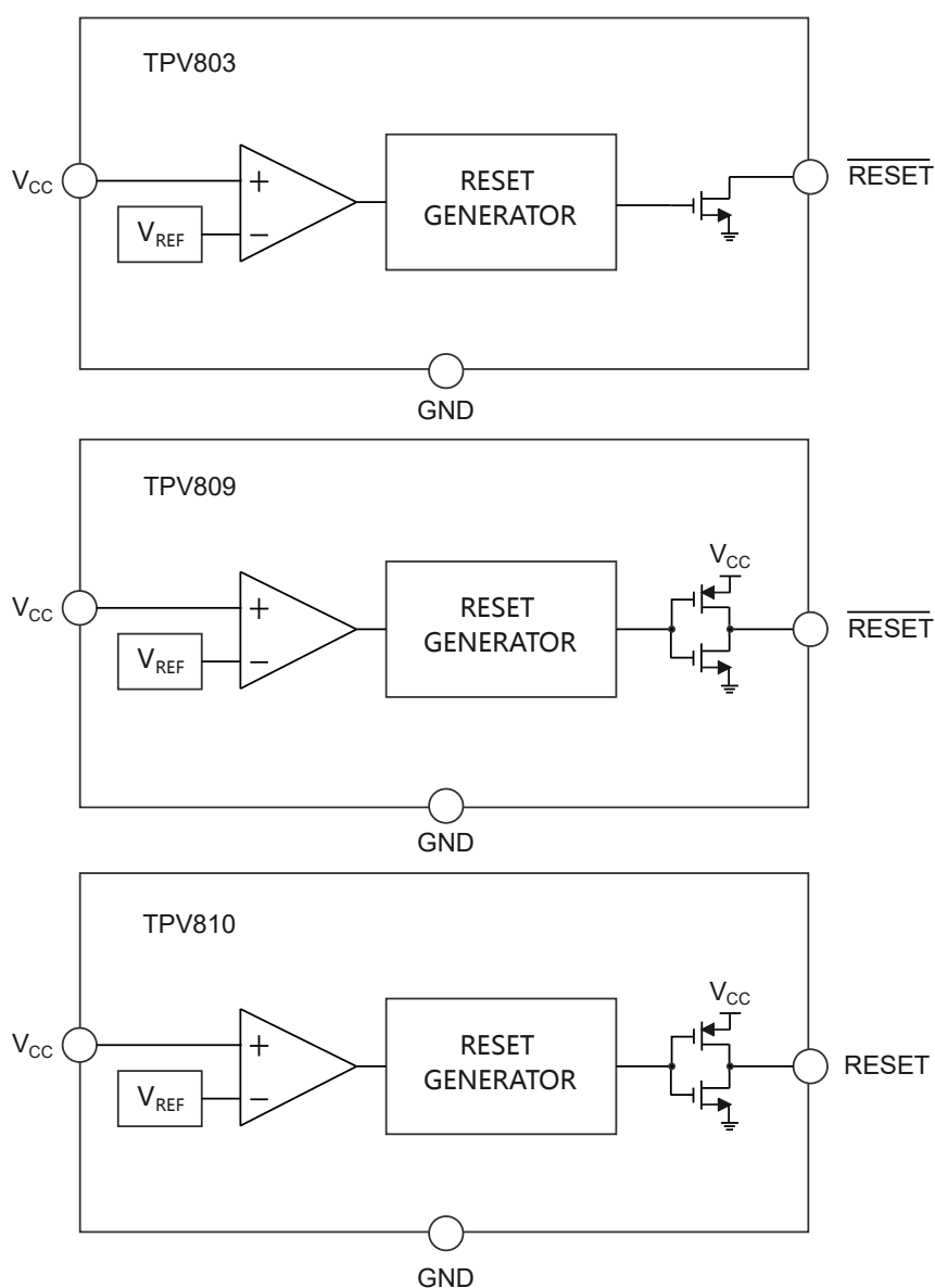
Figure 8. Functional Block Diagram
