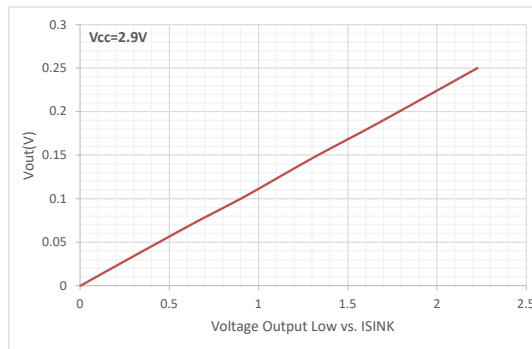
Figure 4. Voltage Output Low vs I_{SINK} (TPV809)
