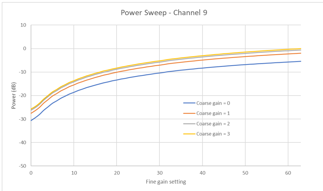
Figure 5: Tx power coarse and fine gain settings Channel 9
