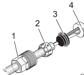
Figure 25 Individual parts
