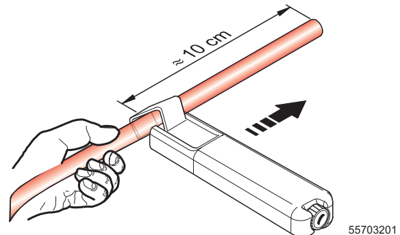
Figure 14 Stripping the outer cable sheath using KAMES LWL
