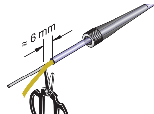
Figure 38 Cutting off the strain relief
