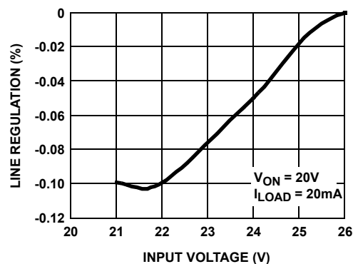
FIGURE 8. V_{ON} LINE REGULATION
