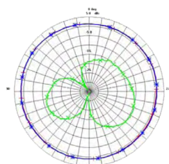
Azimuth 2.45 GHz
