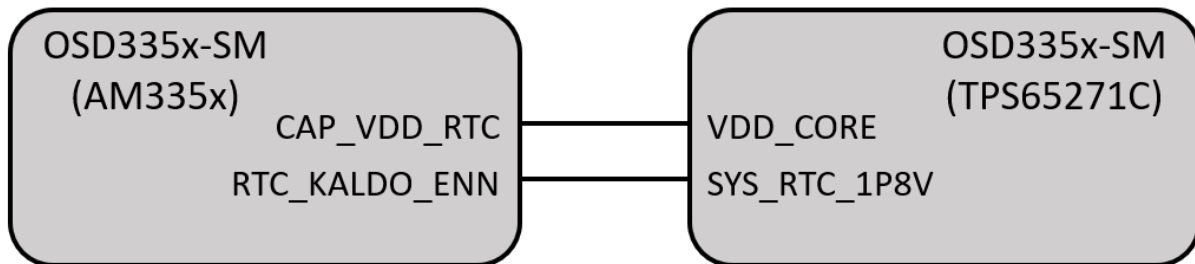
Figure 7.4. Additional connections for OSD335x-SM with RTC disabled
