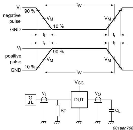
Test data is given in Table 9 . Definitions for test circuit: R_T = Termination resistance should be equal to output impedance Z_o of the pulse generator; C_L = Load capacitance including jig and probe capacitance.
