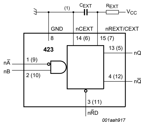
(1) For minimum noise generation it is recommended that the nCEXT pins (6, 14) are connected to ground externally to the GND pin (8).
