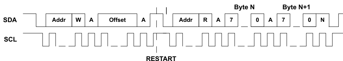
Figure 51. I²C Read Operation
