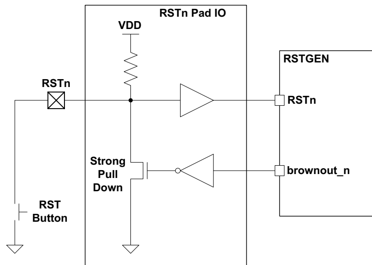
Figure 86. Block diagram of circuitry for Reset pin
