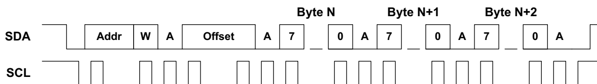
Figure 28. I²C Write Operation with Address Offset
