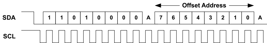
Figure 49. I²C Offset Address Transmission
