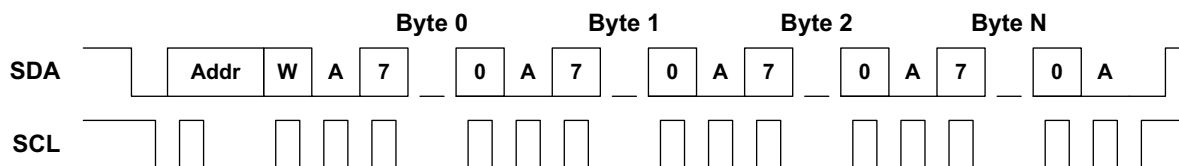
Figure 30. I²C Write Operation with No Address Offset
