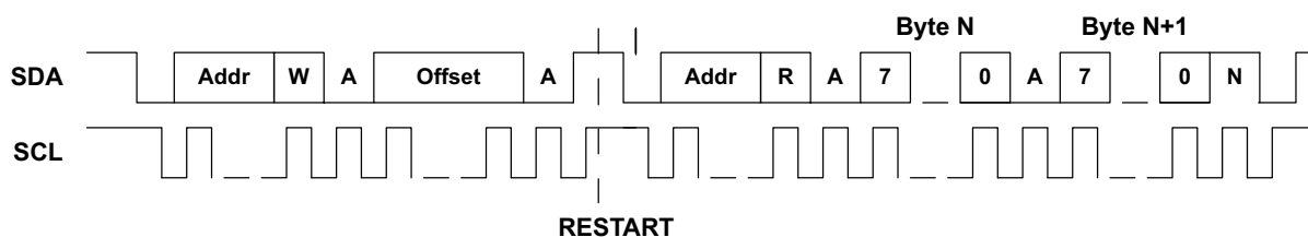
Figure 29. I²C Read Operation with Address Offset
