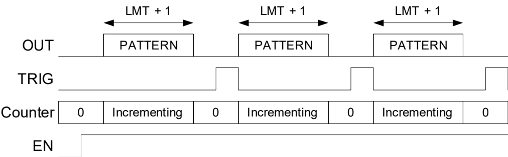
Figure 75. Triggered One-Shot Patterns
