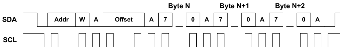
Figure 50. I²C Write Operation
