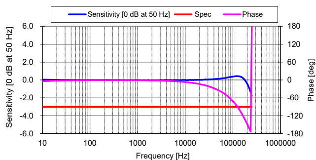
Figure 7: Frequency response
