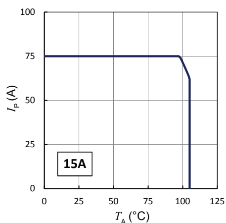
Figure 17: I_p vs T_A for HO series
