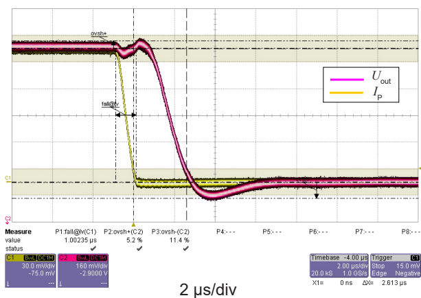
Figure 8: Step response
