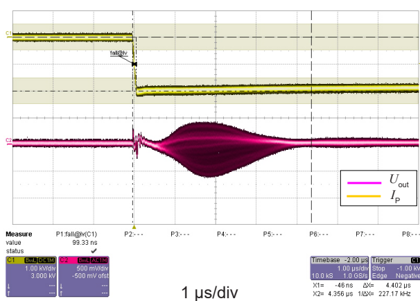
Figure 9: dv/dt
