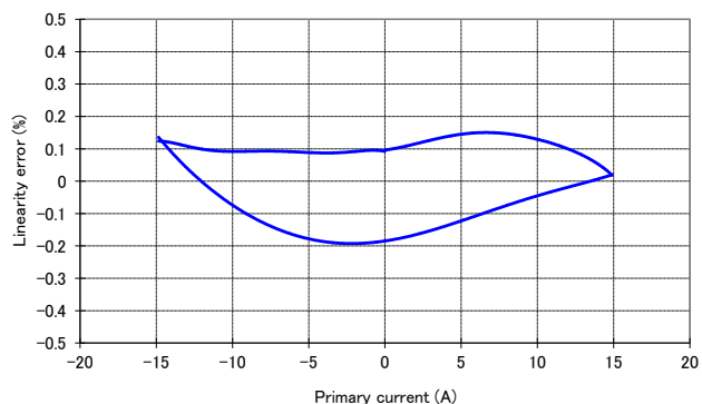
Figure 6: Linearity error
