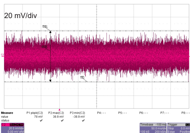
Figure 5: Output noise
