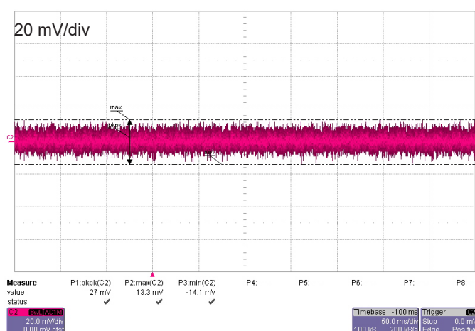
Figure 15: Output noise
