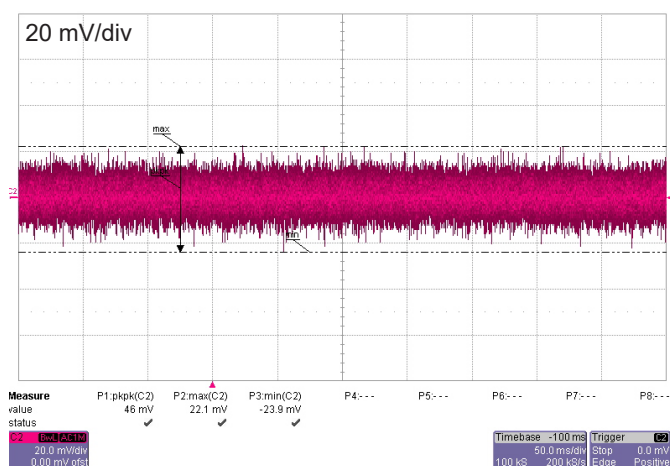
Figure 10: Output noise
