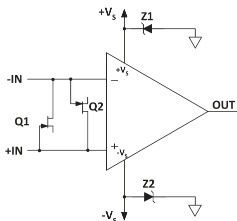
Figure 19: Overvoltage Protection
