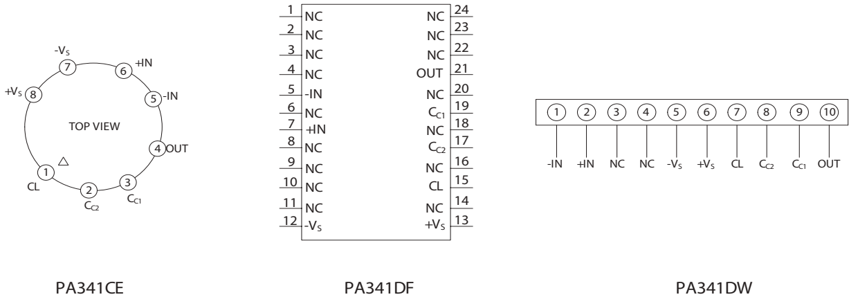
Figure 3: External Connections
