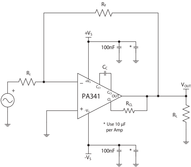
Figure 2: Typical Connection
