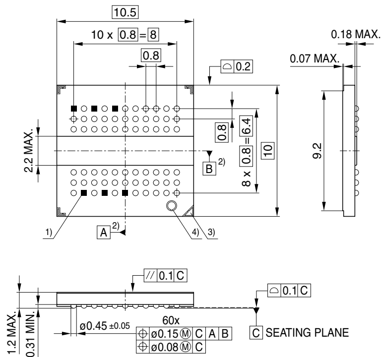
FIGURE 11 Package Outline PG-TFBGA-60
