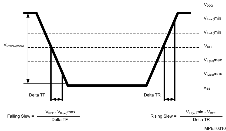
FIGURE 4 Single-ended AC Input Test Conditions Diagram
