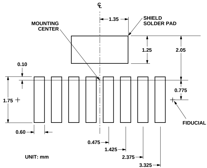
Figure 15. Land pattern.
