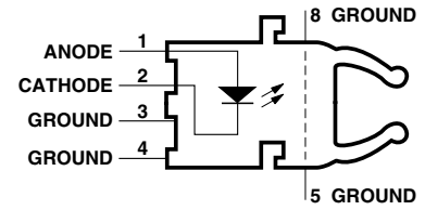
HFBR-1528 Transmitter, Top View
