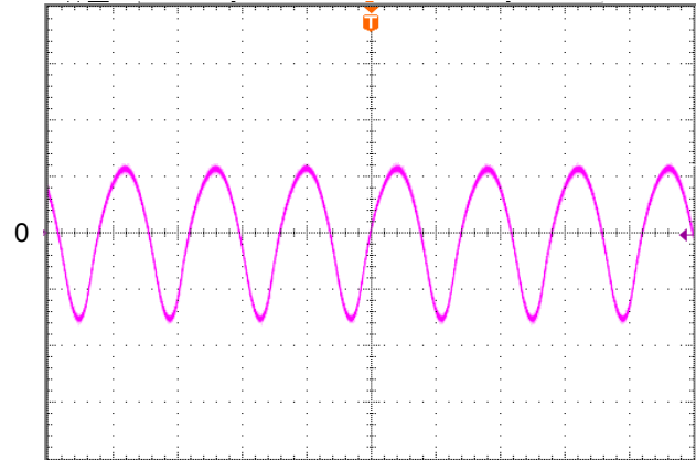
Figure 9: Input Terminal Ripple Current, i_c , at full rated output current and nominal input voltage ( V_{in}=48V ) with 12 \mu H source impedance and 33\mu F electrolytic capacitor (250mA/div, 2us/div)
