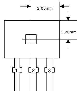
Sensor Location
