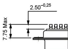
Solder Buckets
