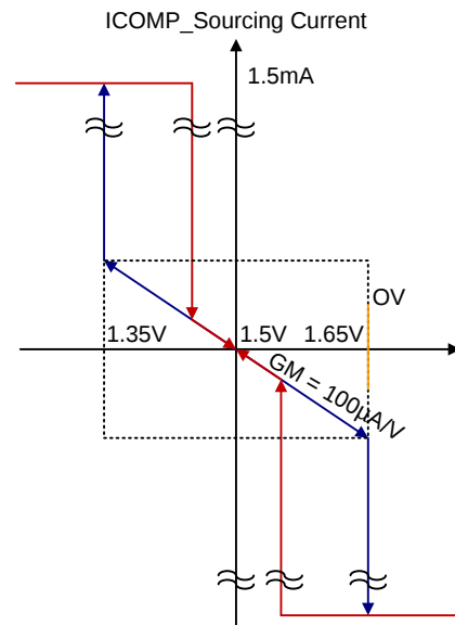
Figure 6. Non-linear GM
