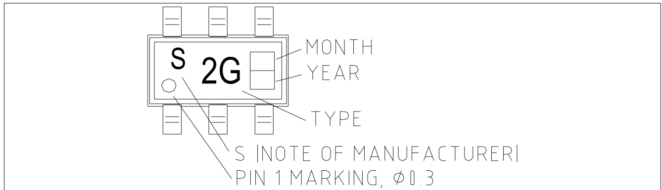
Figure 5 Marking PG-TSOP6-6-9
