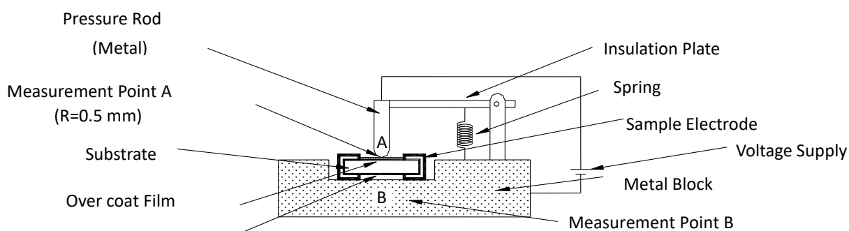
Figure 1 : Measurement Setup
