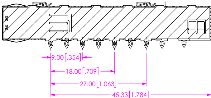
SECTION "A"- "A" SCALE 1.5 : 1
