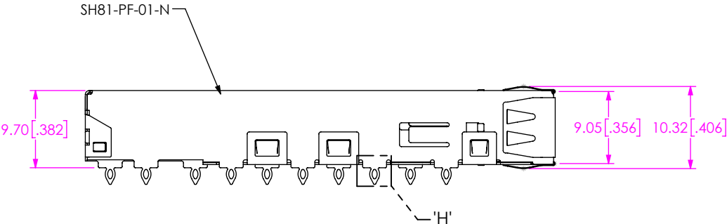
FIG 7 QSFP-1-1-S-N-F SHOWN (SAME AS FIG 1, EXCEPT AS SHOWN)
