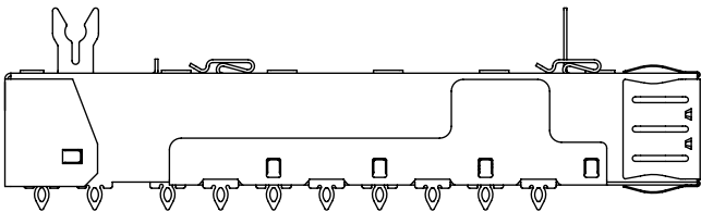
FIG 6 QSFP-C-1-2-S-LP-F SHOWN (DIFFERENT AS SHOWN, OTHERWISE SAME AS FIG 3 & 4)
