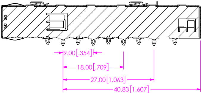
SECTION "B"- "B" SCALE 1.5 : 1
