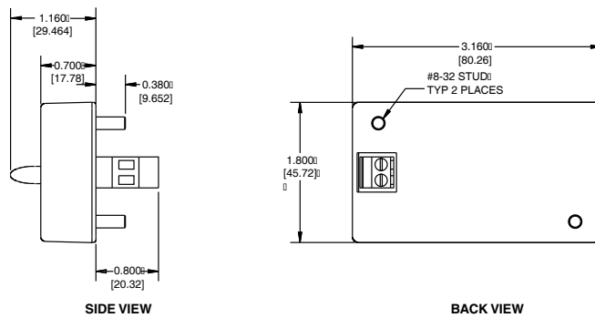
CRM2000 - R UNIT DIMENSIONS
