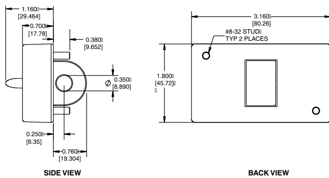
CRM2000 - I UNIT DIMENSIONS
