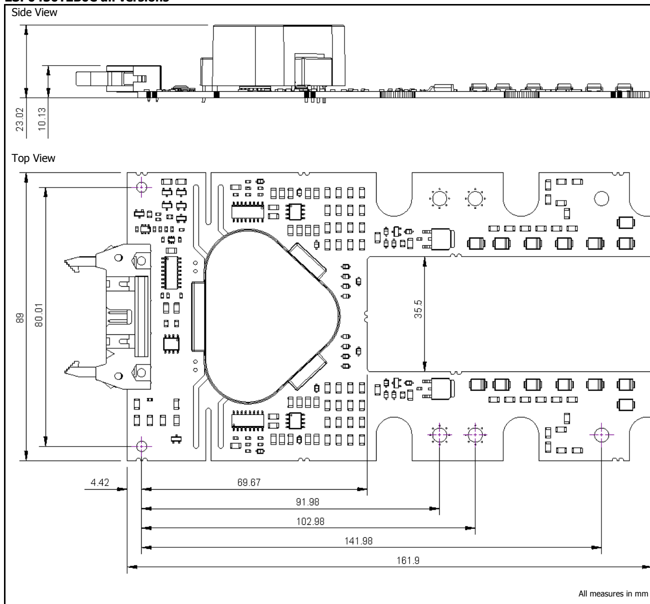
Figure 10. Dimensions.
