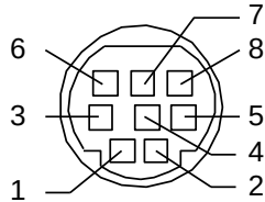
Mini-Din 8 female, front view
