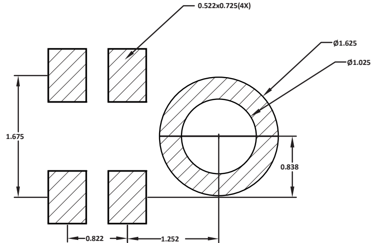
Figure 14. Recommended PCB Land Pattern Layout
