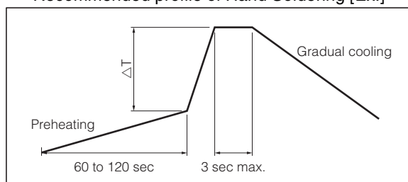
<Allowable temperature difference \Delta T >
