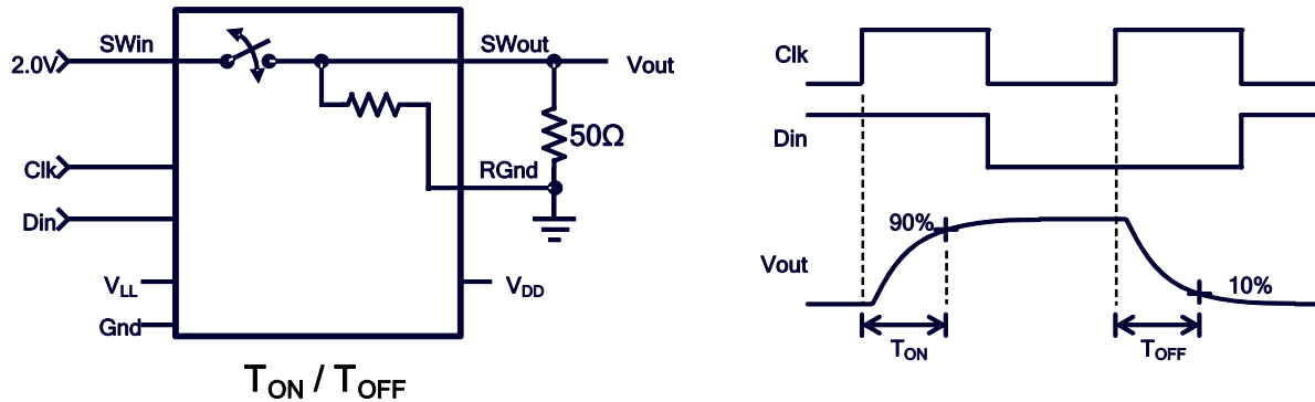
Test Circuit 5
