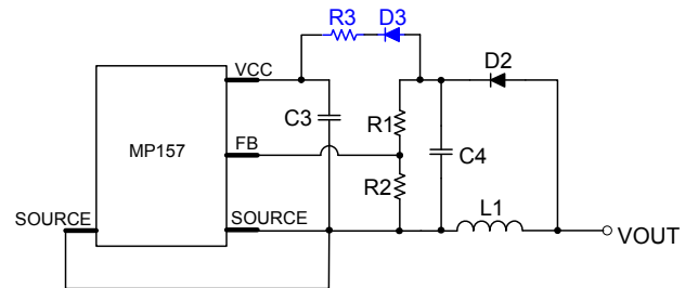
Figure 9: Auxiliary V_{\text{CC}} Supply Circuit
