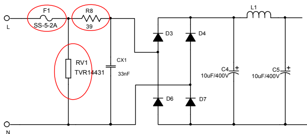
Figure 10: Solution to Pass 2kV Surge Test Layout Guide
