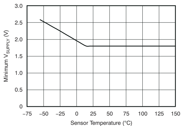
Figure 6-8. Minimum Supply Voltage vs Temperature
