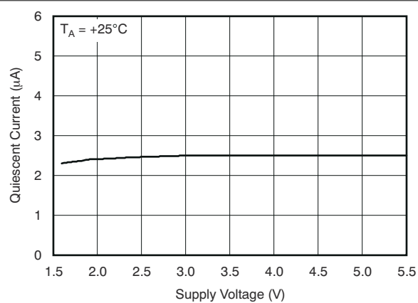
Figure 6-4. Quiescent Current vs Supply Voltage
