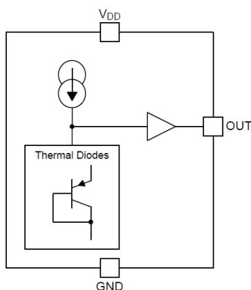
Device Block Diagram
