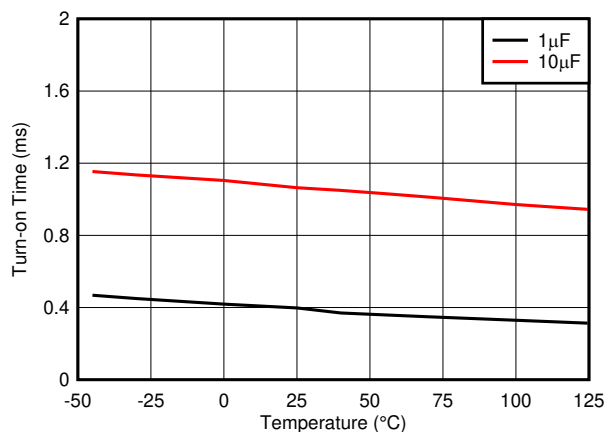
Figure 10-4. REF70 Turn-on Time
