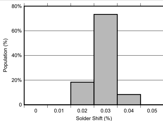
Figure 8-2. Solder Shift (LCCC Package)
